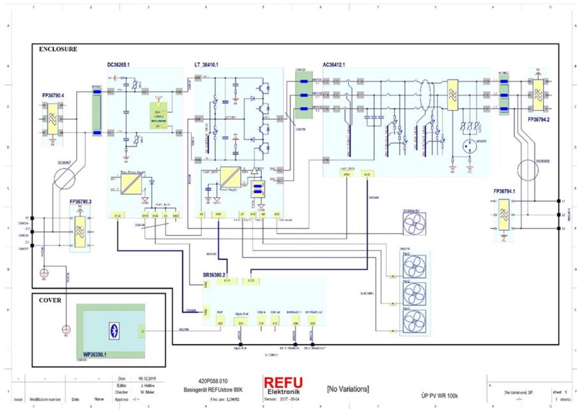
Figure 3 – Block diagram of the battery inverter
