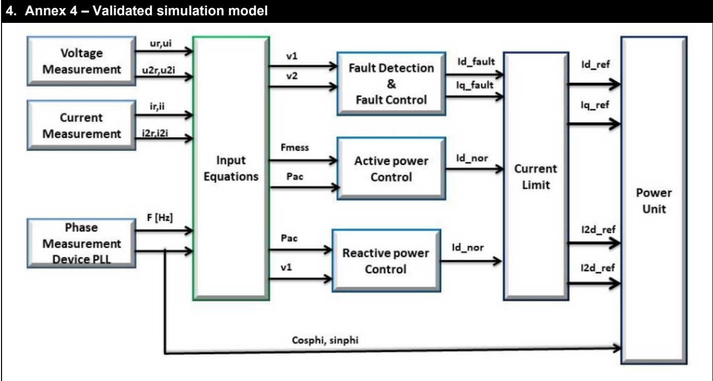
Figure 20 – Control frame of the simulation model
