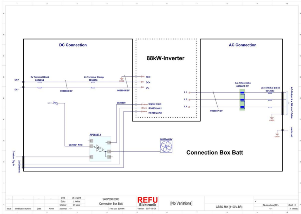
Figure 4 – Block diagram Connection boxes
