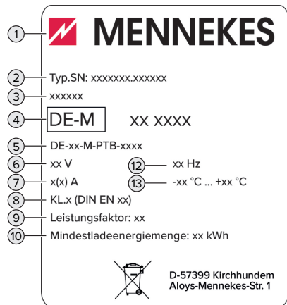
Abb. 1: Eichrecht-Typenschild (Muster)
